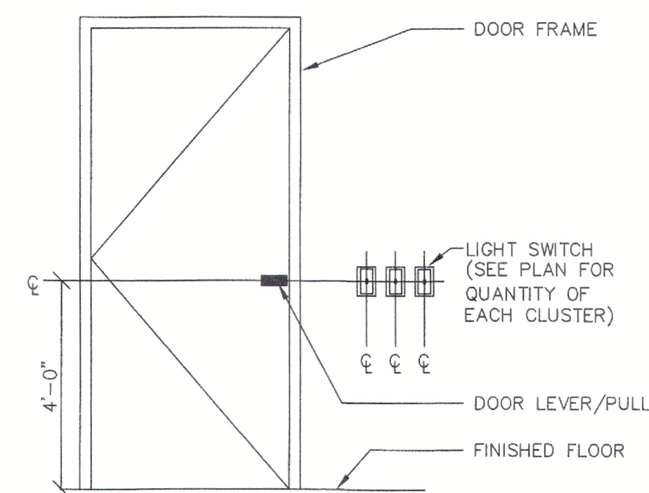
TYPICAL LOCATION FOR LIGHT SWITCHES. NTS
