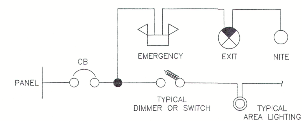
TYP. EMERGENCY LIGHT WIRING DIA.
